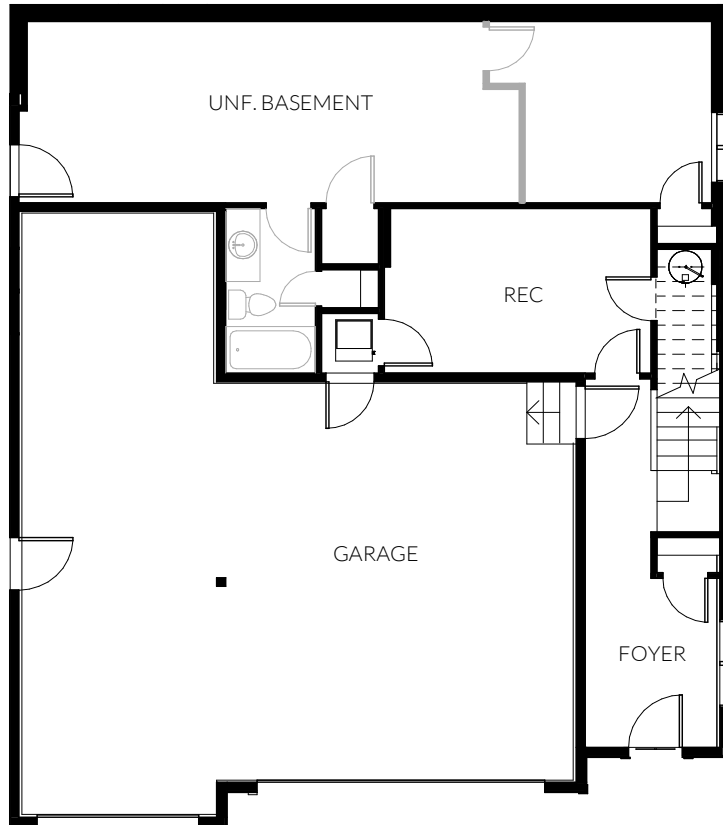
BASEMENT 927 SQ. FT. GARAGE 876 SQ. FT.
